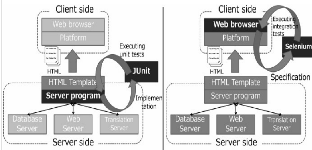
Figure 6.1: Testing Workflow
